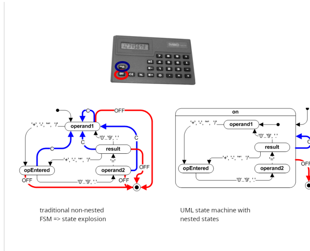
Figure 4.3: hierarchical states calculator example
