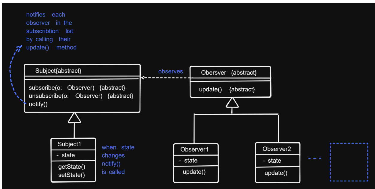
Figure 4.11: observer pattern
